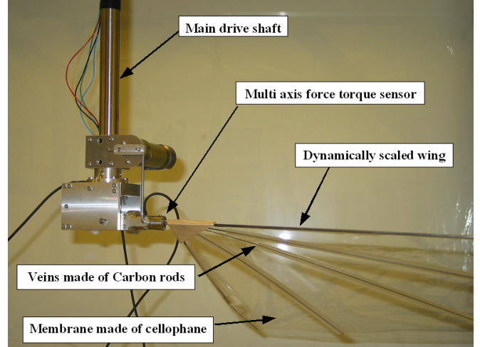
Fig. 4. Figure shows the robotic flapper designed and fabricated at University of Delaware. It is driven by three independent servo motors and can give 3-DOF flapping wing motion. A six-axis force torque sensor (Nano 17) from ATI industrial automation is mounted at the base of the wing.
