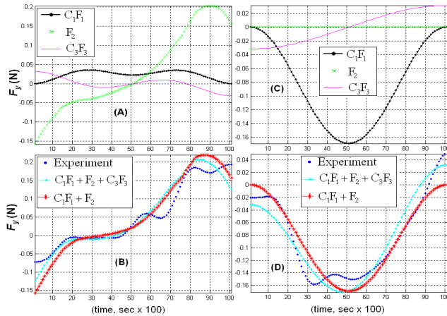
Fig. 8. Comparison of F_y component of total aerodynamic force F_T = C_1F_1 + F_2(C_1, C_2) + C_3F_3 . (A) and (B) shows the comparison for the pattern having amplitudes \Phi = 46^\circ , \Psi = 74.9^\circ , (C) and (D) shows the comparison for the pattern having amplitudes \Phi = 46^\circ , \Psi = 0^\circ .
