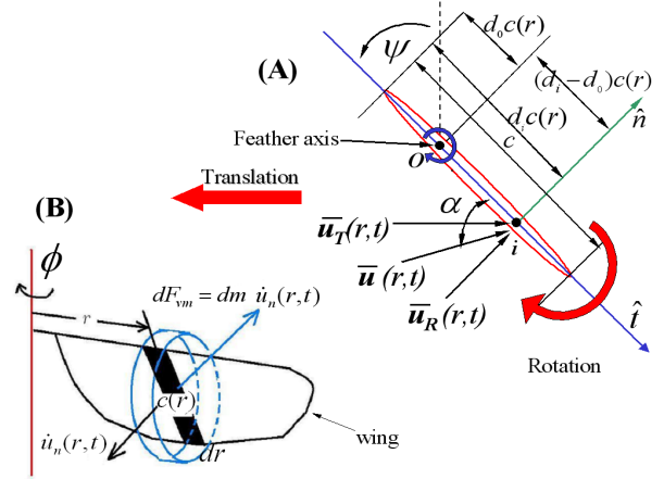
Fig. 3. (A) The combined rotational and translational/LEV effect on a wing section. (B) Virtual mass force acting at a section.
