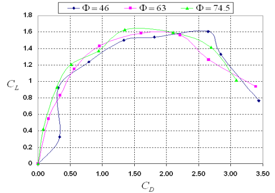
Fig. 7. Lift and drag polar plot for three stroke amplitudes, i.e., \Phi = 46^\circ, 63^\circ, 74.5^\circ . These coefficients are computed at the mid-stroke position during the flapping cycle similar to the determination of C_1 .
