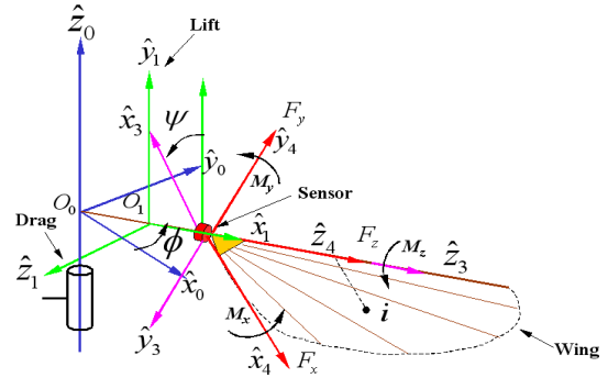
Fig. 4. Figure shows the robotic flapper designed and fabricated at University of Delaware. It is driven by three independent servo motors and can give 3-DOF flapping wing motion. A six-axis force torque sensor (Nano 17) from ATI industrial automation is mounted at the base of the wing.
