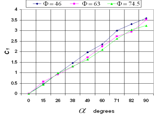
Fig. 6. Coefficient of LEV/translational force C_1 Vs \bar{\alpha}
