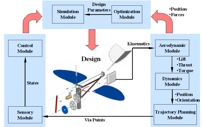
Fig. 1. The architecture of FW-MAV Design
