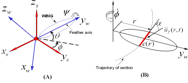
Fig. 2. (A) Wing angles ( \phi, \theta, \psi ). (B) Translational motion
